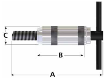
TYPE IV Non-Captive Prewinder
